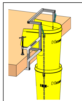
SUPPORT DALLE Code 318103501
