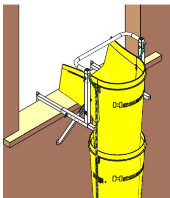
SUPPORT FENETRE Code 318103201
