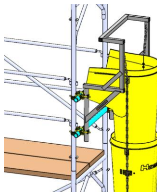
SUPPORT ECHAFAUDAGE Code 318104501
